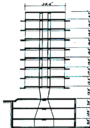
ATLANTIC BUILDING CROSS SECTION - LOOKING SOUTH
